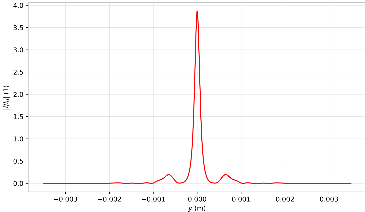
Intensity profile I(x=0, y, z=1.194)/I_0 , \text{Pin}=9.0\text{Pcr} , artificial time
